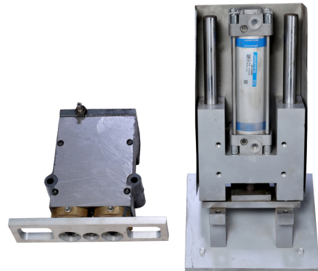
PUSHER ASSEMBLY, GOB INTERCEPTOR
